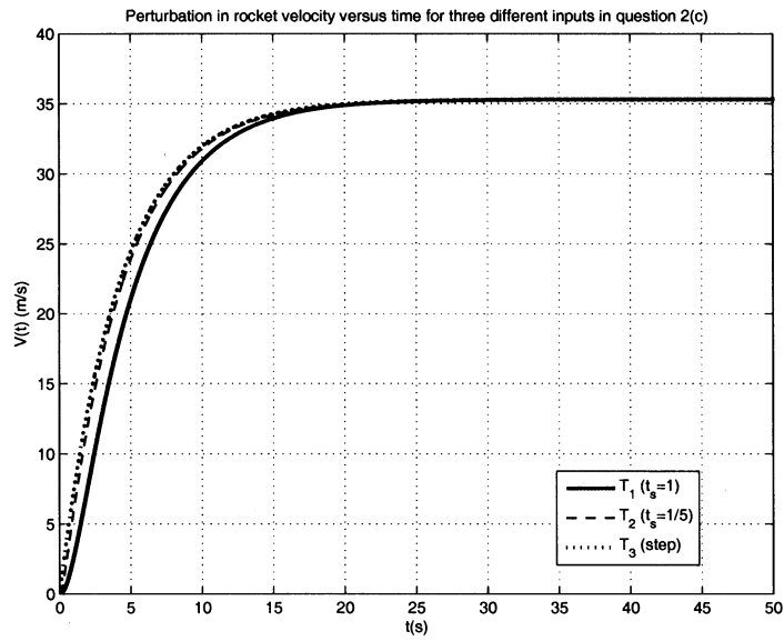
Figure 3: Velocity perturbation response of rocket with three different inputs: T'_1(t) = (1 - e^{-t})\sigma(t) , T'_2(t) = (1 - e^{-5t})\sigma(t) , and T'_3(t) = \sigma(t) .
